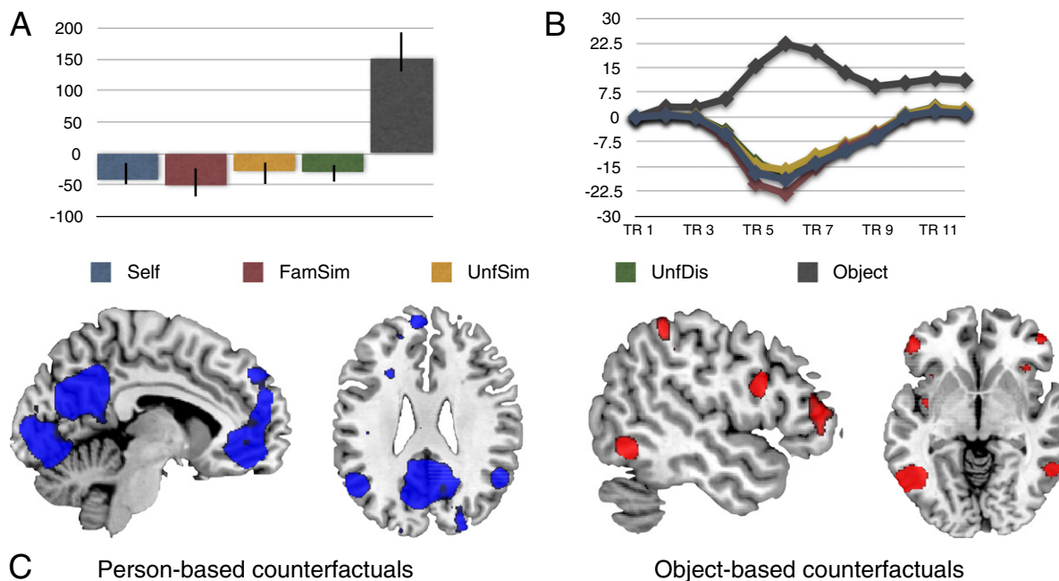
Fig. 2. Results from mean-centered PLS analysis: Latent Variable 1 (LV1). (A) Plot of brain scores with confidence intervals. (B) Plot of temporal brain scores indicating weighed average of activation across all voxels in all participants during the length of the task. (C) Regions with negative saliences (blue) were engaged by person-based counterfactuals, whereas regions with positive saliences (red) were engaged by object-based counterfactuals. All regions are shown at a threshold of p < .001 .
